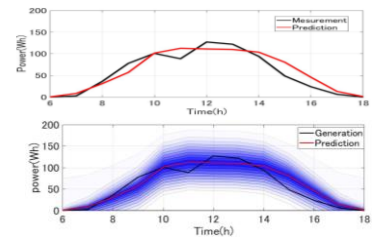
PV power prediction
