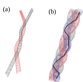
Fig. 5 Schematic representations of optical branching device (a) double helix type and (b) triple helix type [1] .
