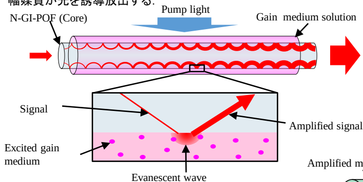
Fig. 1 Principle of evanescent wave optical amplifier.
