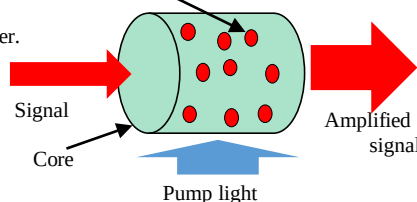
Fig. 3 Principle of fluorescent substance doped optical amplifier.
