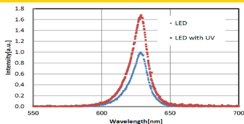
Fig. 2 Spectra of signal and amplified signal [3] .
