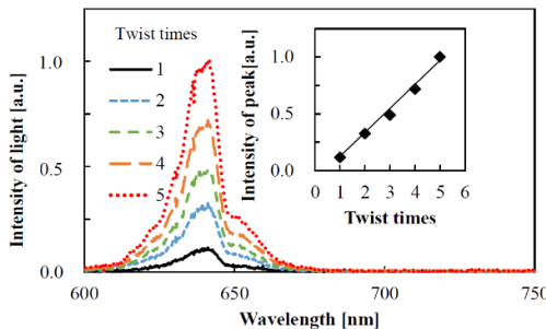
Fig. 6 Output spectra and peak intensities of branched output light [1] .
