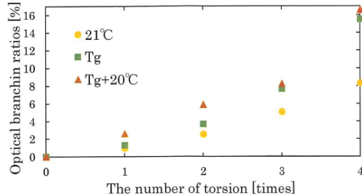
Fig. 7 Comparison of the optical branching ratios among different contact treatment temperatures [4] .
